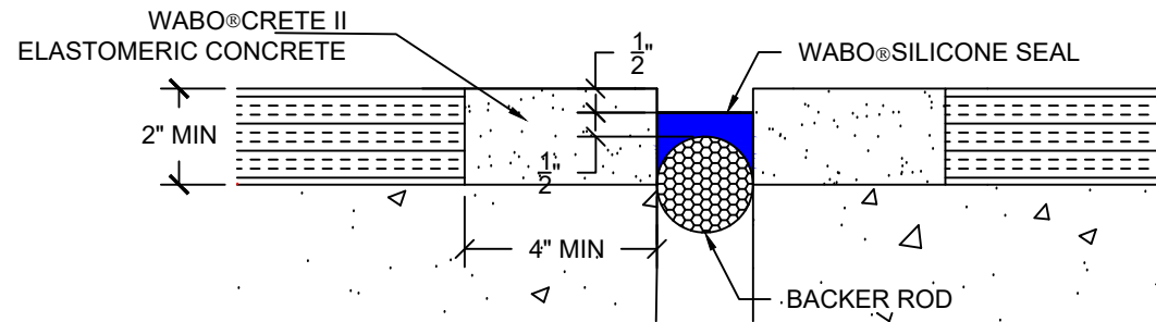
ELASTOMERIC CONCRETE CONDITION
