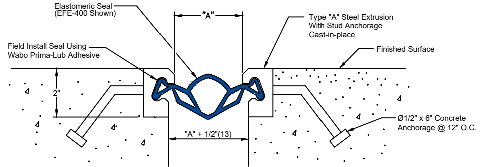
Wabo® StripSeal (Model:SSS, Type A) DETAIL SLAB TO SLAB CONDITION NOT TO SCALE
