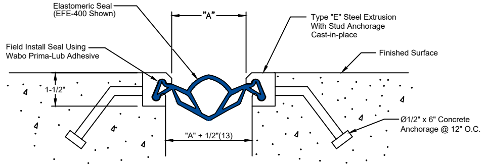
Wabo® StripSeal (Model:SSS, Type E) DETAIL SLAB TO SLAB CONDITION NOT TO SCALE
