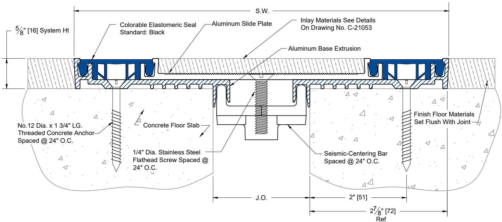
Typical Section Floor To Floor
