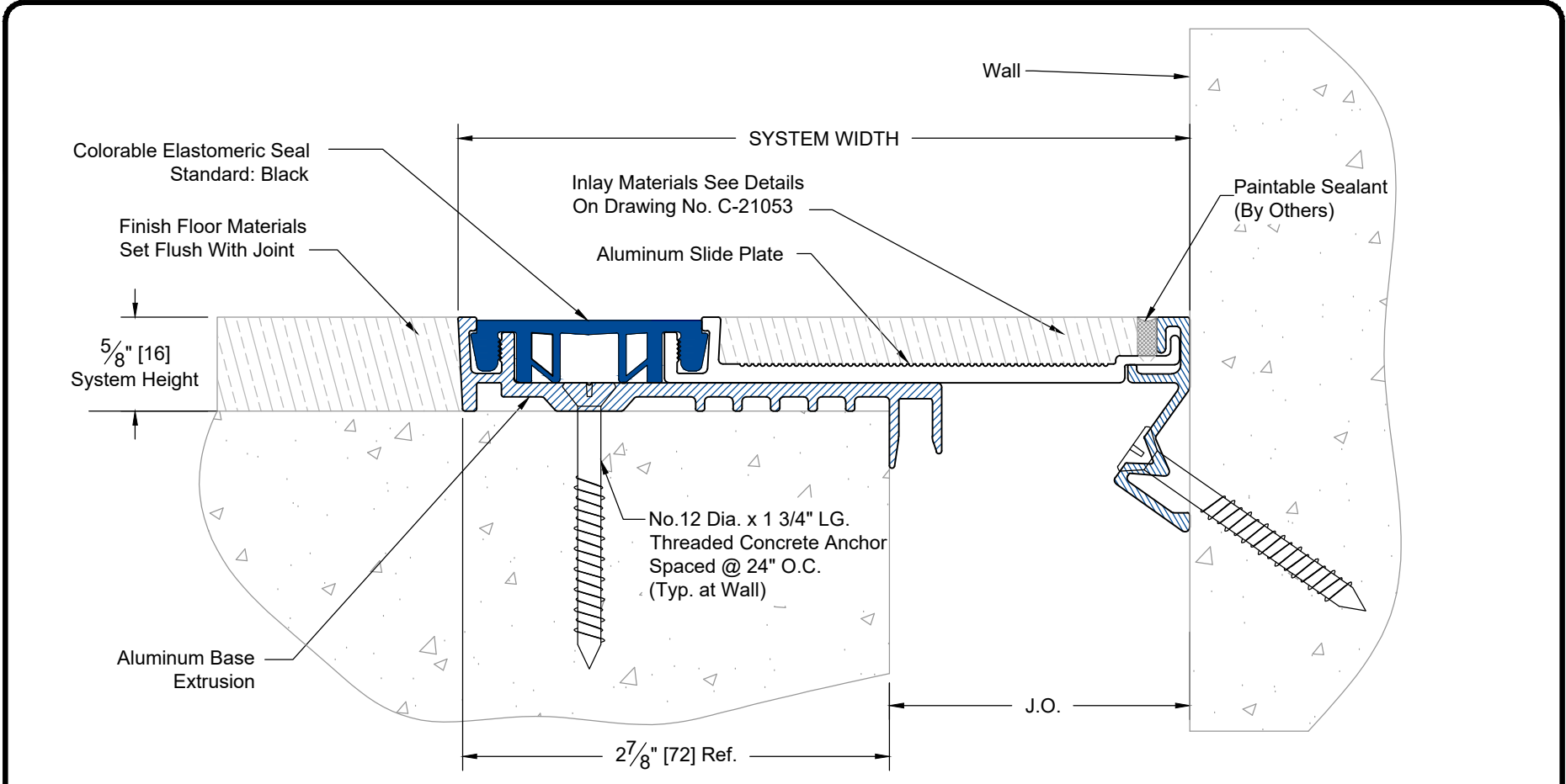
Typical Section Floor To Wall
