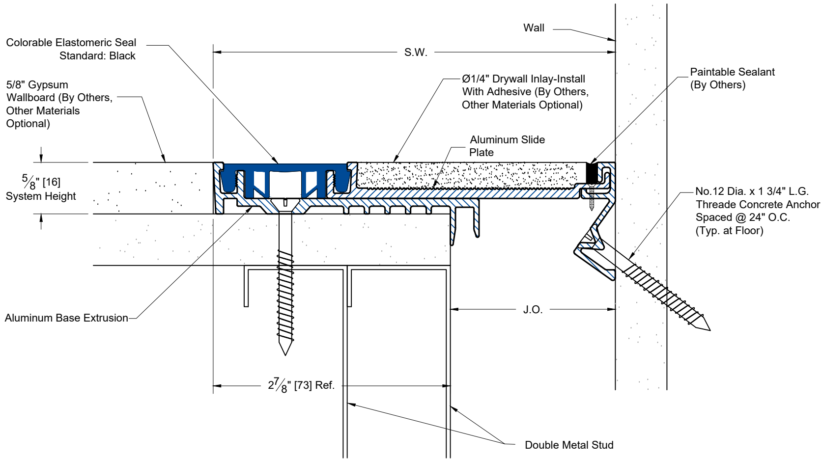
Typical Section
