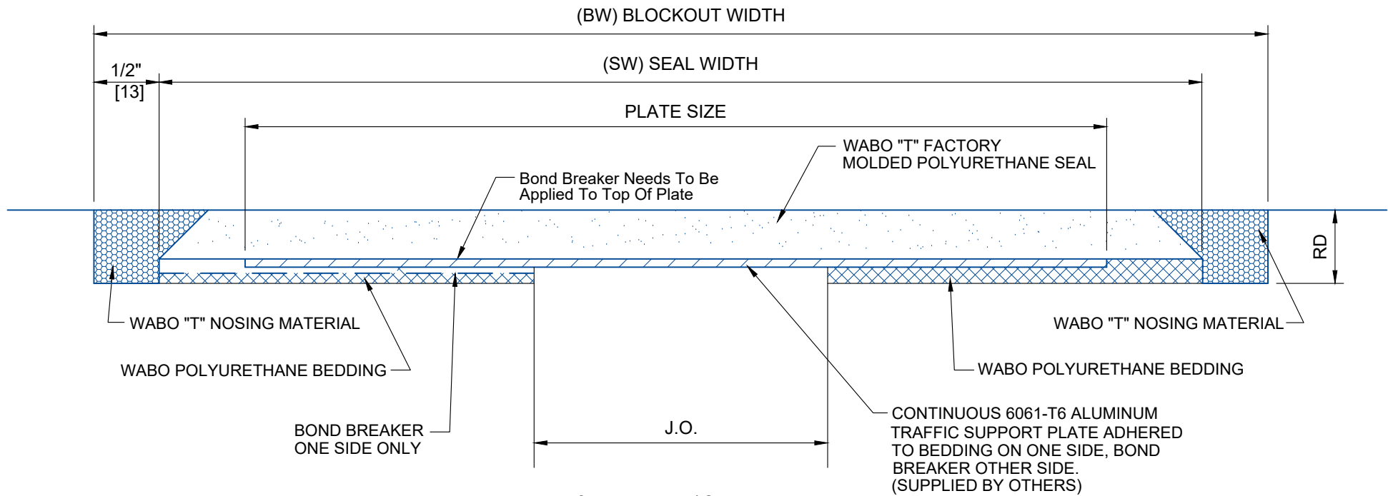
T-3 THRU T-12 DETAIL SLAB-TO-SLAB CONDITION
