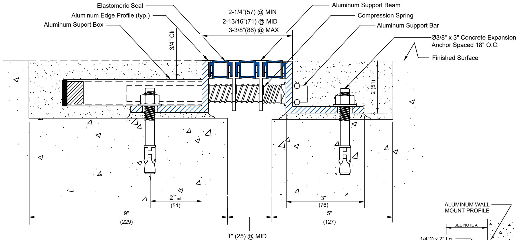
VIP-1125 DETAIL FLOOR-TO-FLOOR CONDITION
