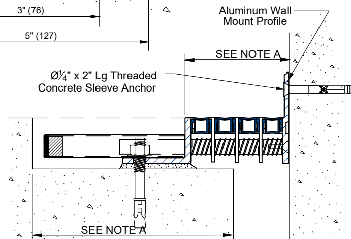
VIP-1500C DETAIL FLOOR-TO-WALL CONDITION
