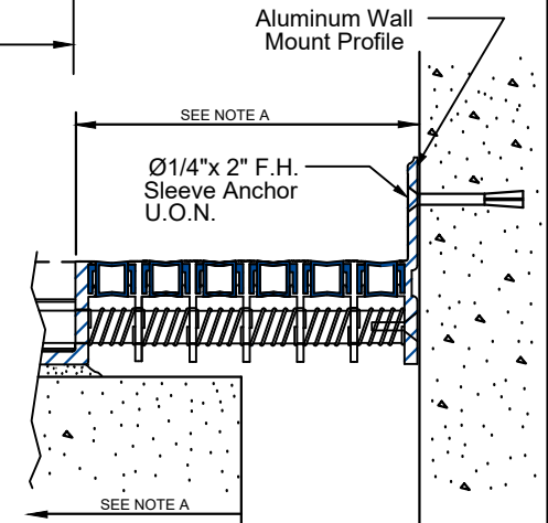
VIP-2250C DETAIL FLOOR-TO-WALL CONDITION
