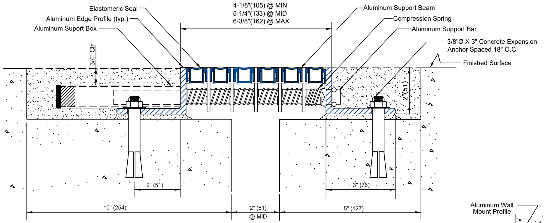
VIP-2250 DETAIL FLOOR-TO-FLOOR CONDITION
