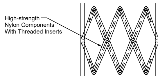
PLAN VIEW PANTOGRAPH CONTROL MECHANISM
