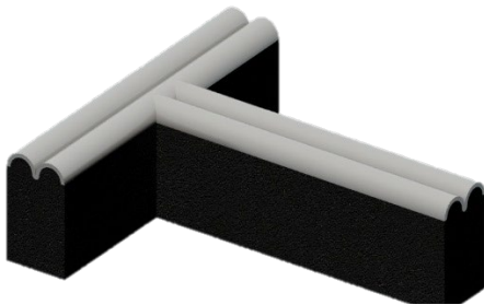
Factory Fabricated "T" Transition
